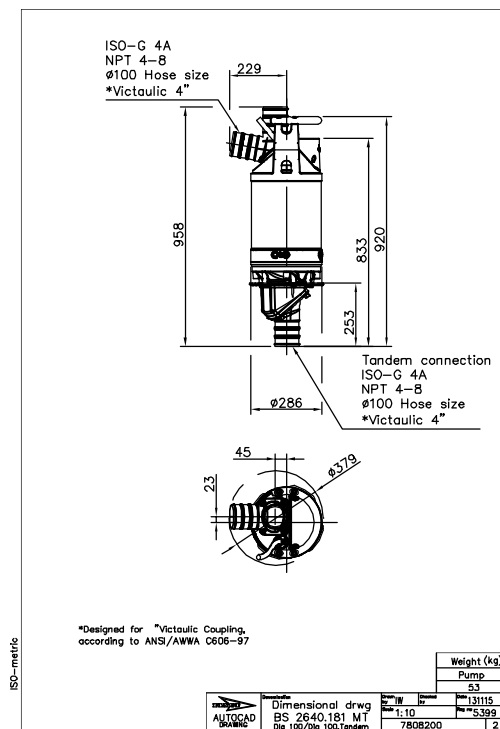
Figura 11: BS, MT, DN 100, tándem
