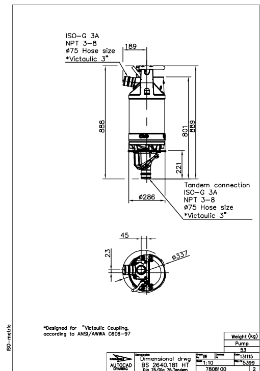
Figura 12: BS, HT, DN 75, tándem
