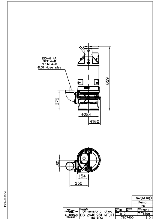
Figura 10: DS, MT/HT, DN 100
