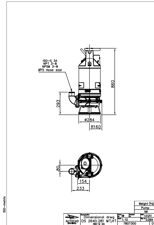
Figura 9: DS, MT/HT, DN 75
