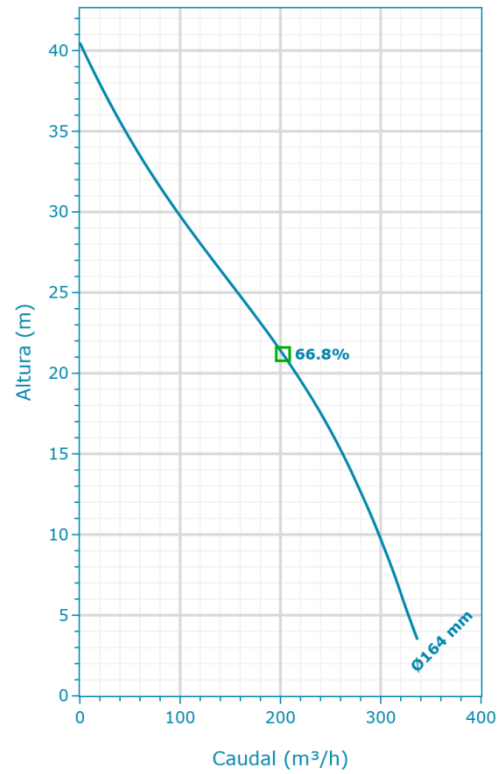
Curve: ISO 9906
